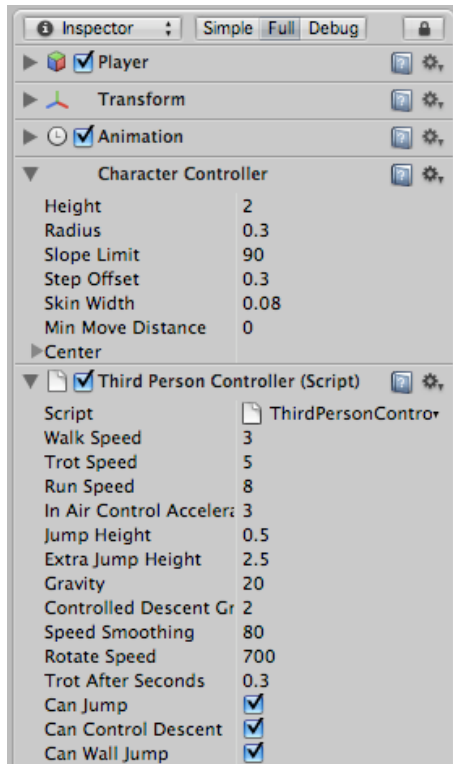
Character Controller and Third Person Controller Script Components in place.
