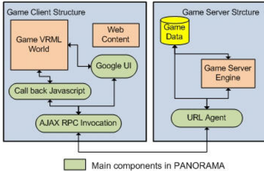
Fig. 2: Architecture PANORAMA (Web)
